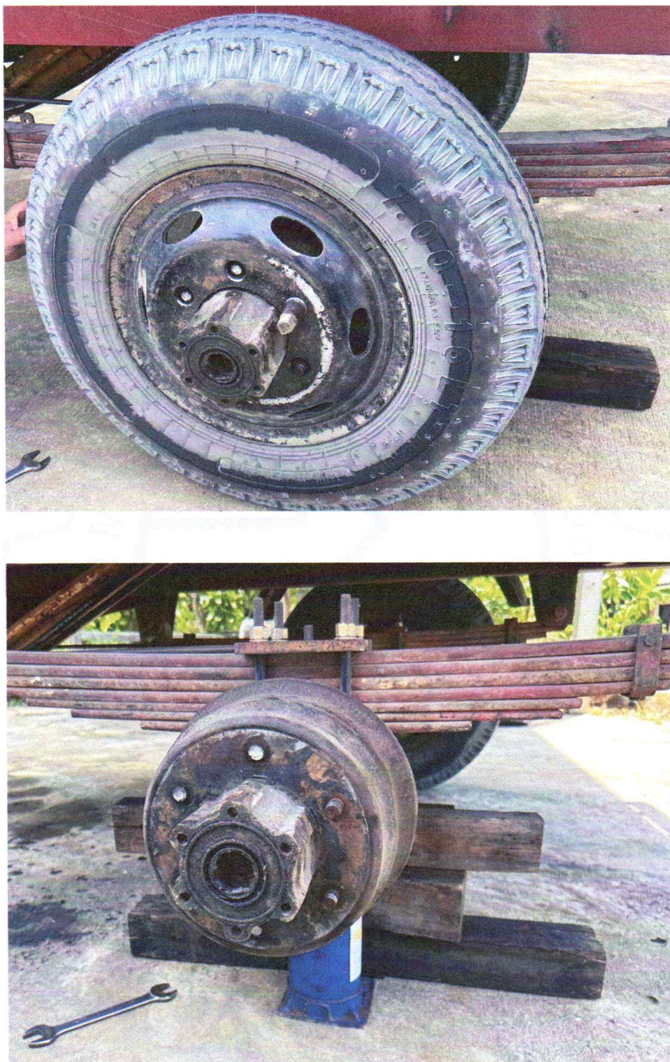
Figure 1. Machine breakdown of SUPER STD-5 Agricultural Trailer during the performance test on paved road.
